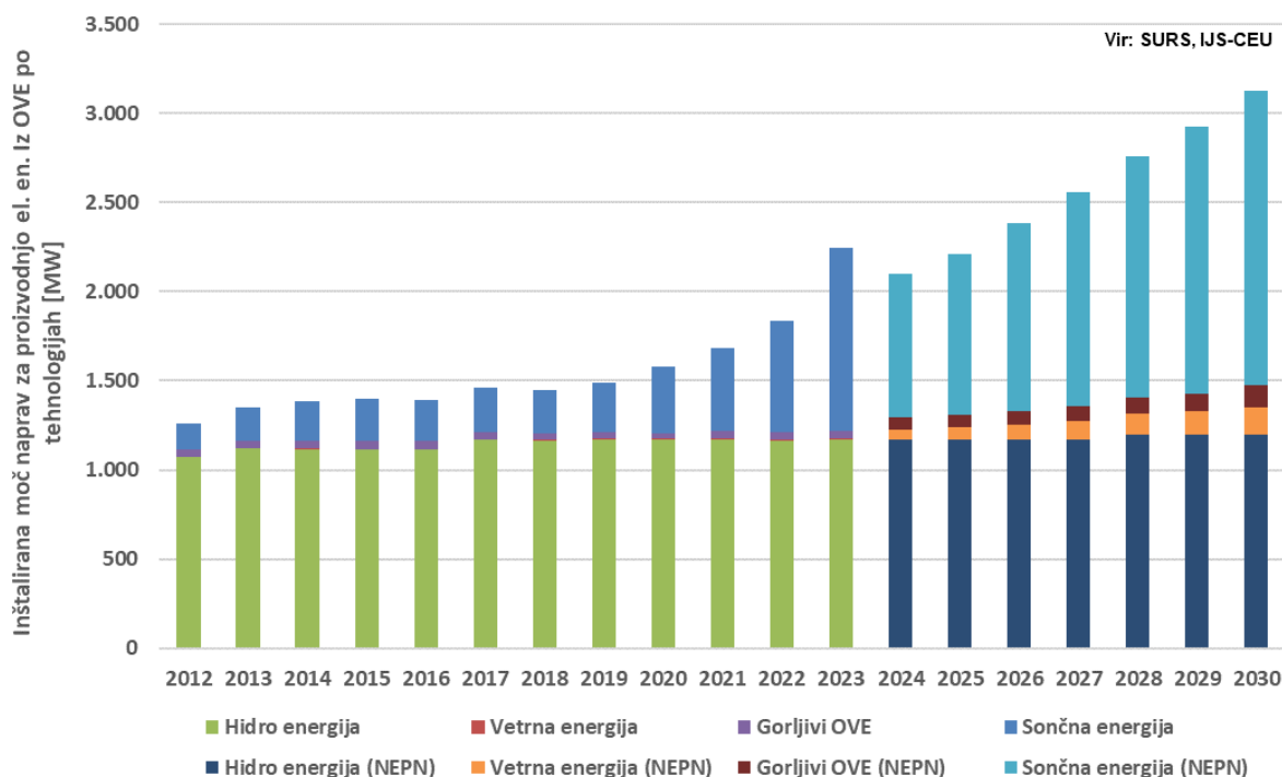
Slika 19: Inštalirana moč naprav za proizvodnjo električne energije iz obnovljivih virov energije po vrsti OVE v obdobju 2012–2023 in letni indikativni cilji iz NEPN za obdobje 2024–2030 (Vir: SURS, IJS-CEU) Installed capacity of the systems for the production of electricity from RES by the RES type in the period 2012–2023 and its annual indicative target values for the period 2024–2030 from NECP (Source: Republic of Slovenia Statistical Office, JSI-EEC)
