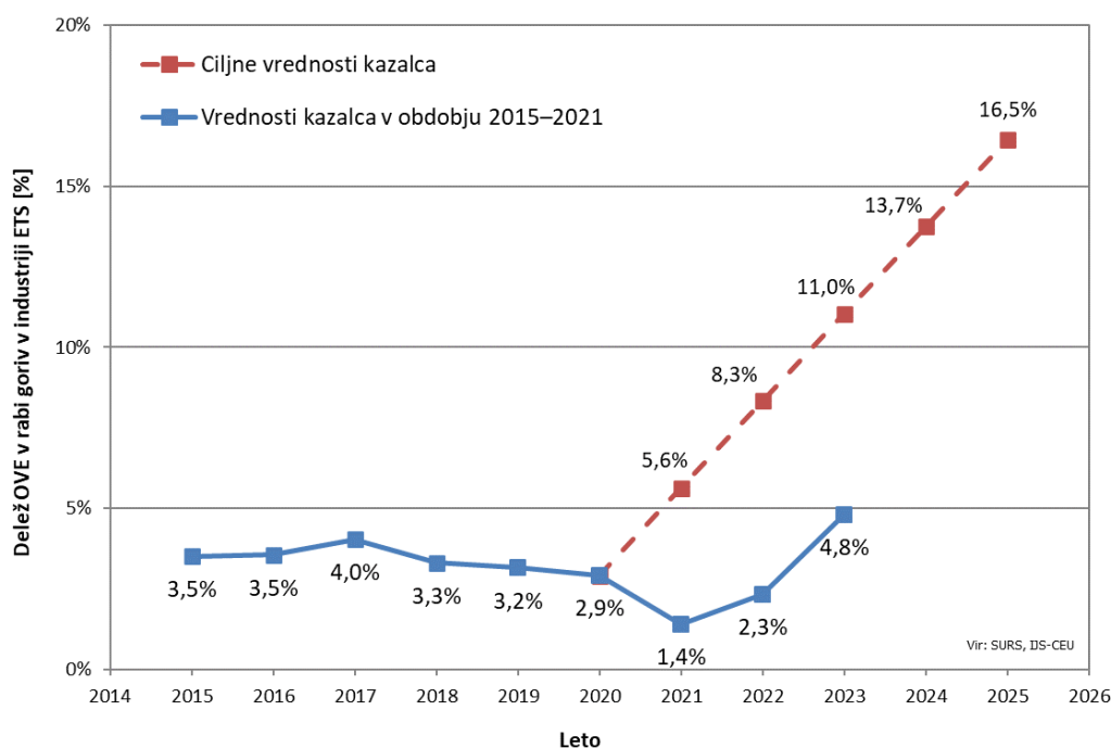
Slika 15: Delež OVE v rabi goriv v industriji ETS v obdobju 2015–2023 ter ciljne vrednosti kazalca do leta 2025 (Vir: SURS, IJS-CEU) The share of RES in the use of fuels in the ETS industry in the period 2015–2023 and its target values up to 2025 (Source: SURS, JSI-EEC)
