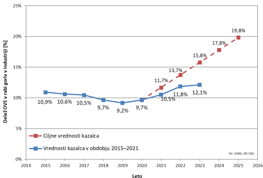
Slika 14: Delež OVE v rabi goriv v industriji v obdobju 2015–2023 ter ciljne vrednosti kazalca do leta 2025 (Vir: SURS, IJS-CEU) The share of RES in the use of fuels in industry in the period 2015–2023 and its target values up to 2025 (Source: SURS, JSI-EEC)
